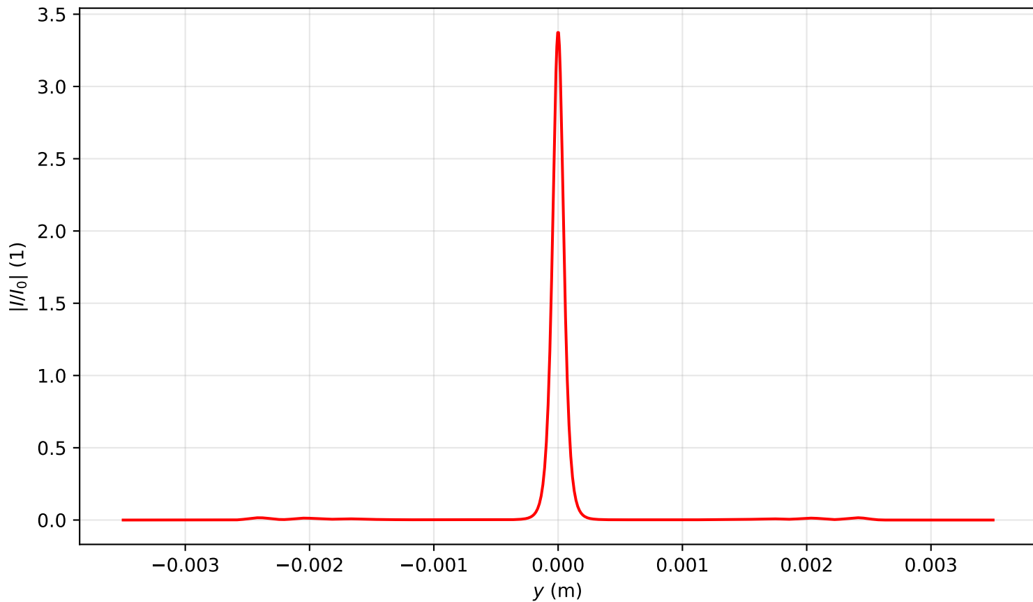
Intensity profile I(x = 0, y, z = 2.388)/I_0 , \text{Pin}=9.0\text{Pcr} , artificial time
